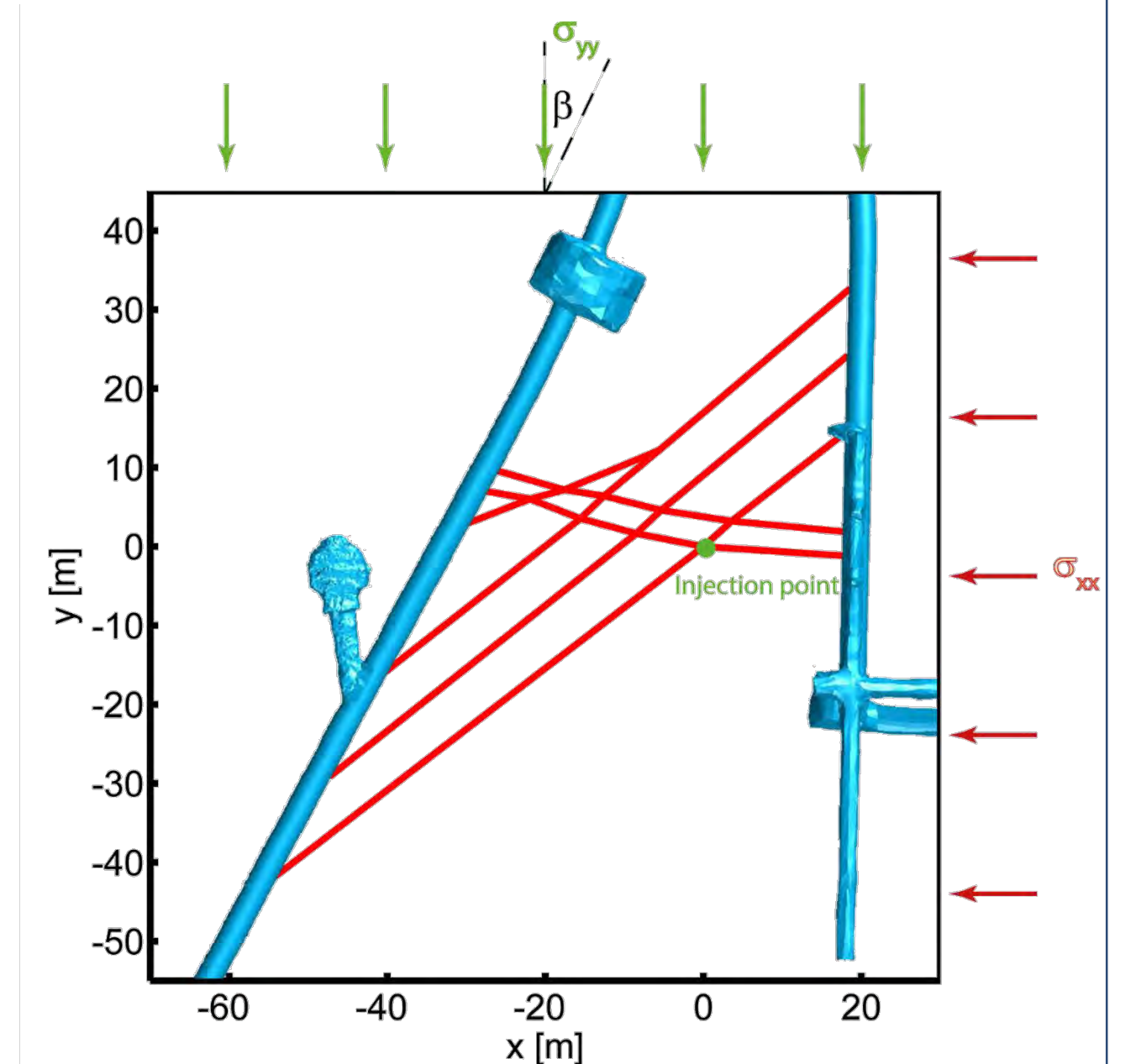
Figure 3. schematic representation of the horizontal cross-section between AU and VE tunnel
