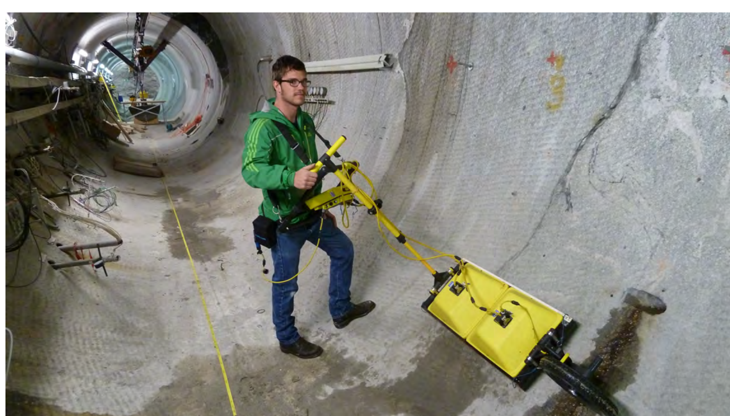
Performing GPR measurements with the PulseEKKO 250 MHz antenna (left) and the MALÅ GX HDR 80 MHz antenna (left)
